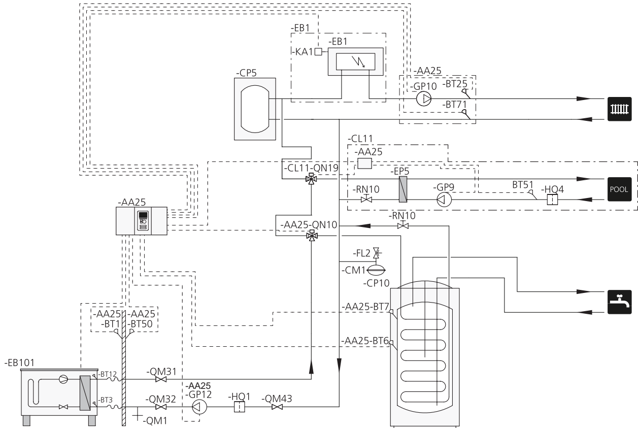
Outline diagram SMO 40 with POOL 40
