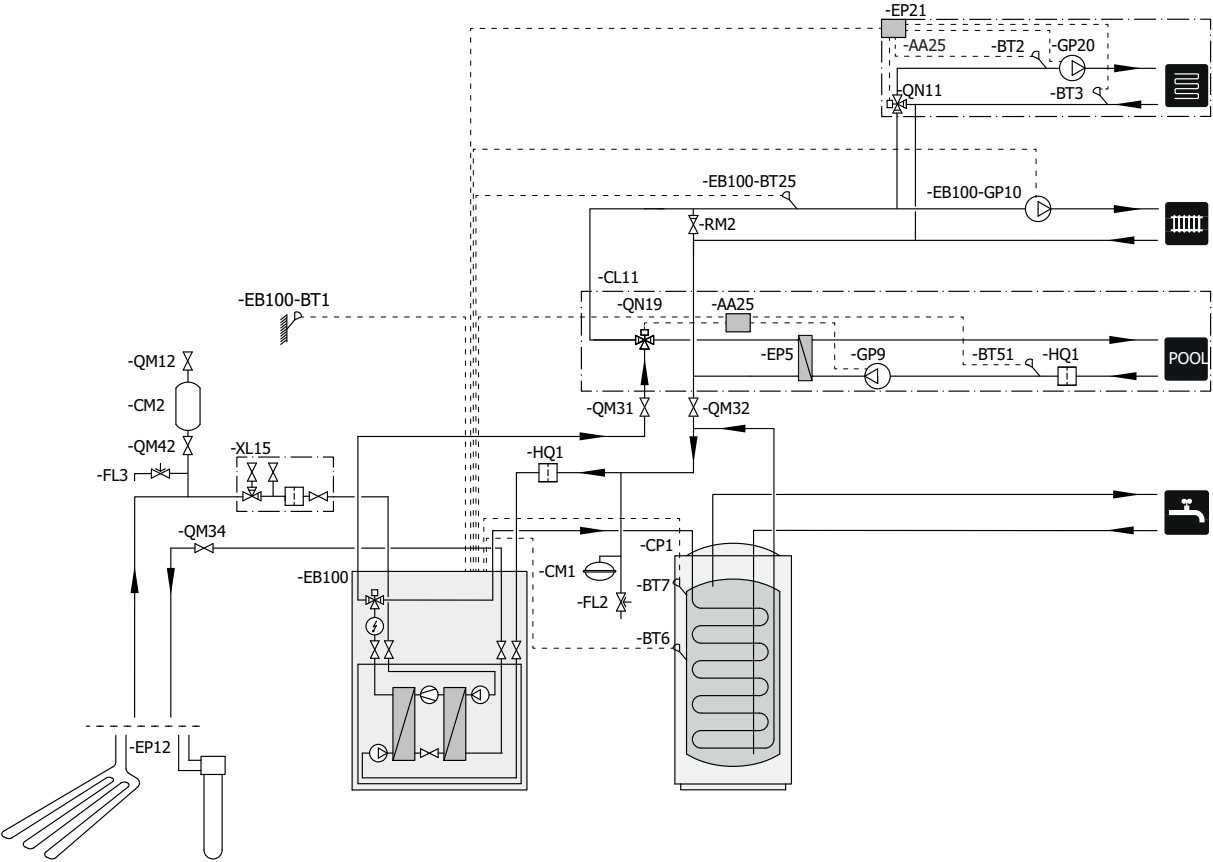
Outline diagram F1145/F1155 with POOL 40 and extra climate system
