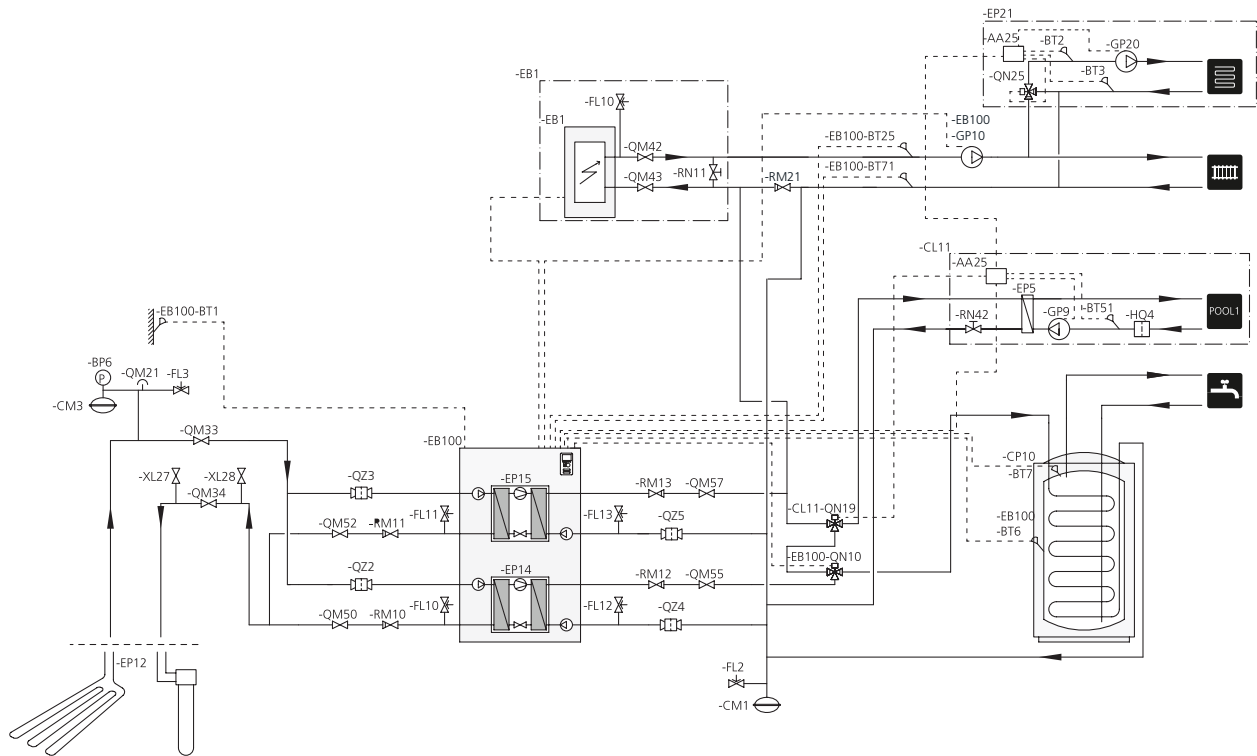
Outline diagram F1355 with POOL 40 and extra climate system
